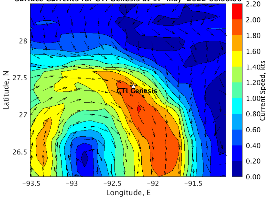
Surface Currents for CTI Genesis at 17-May-2022 00:00:00
